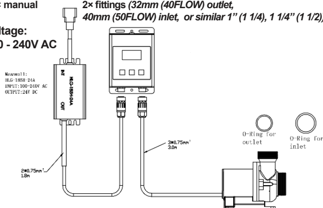
Schematic of connection of the Red Dragon® 5 ECO
