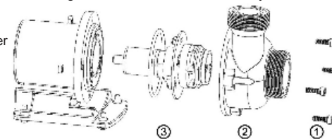
Exploded assembly drawing of the Red Dragon® 5 Eco pump
